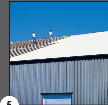
5 Seal entire roof with one of our approved acrylic coatings: • PUMA® XL • Benchmark® • Rapid Roof® III • Rapid Roof® HV
